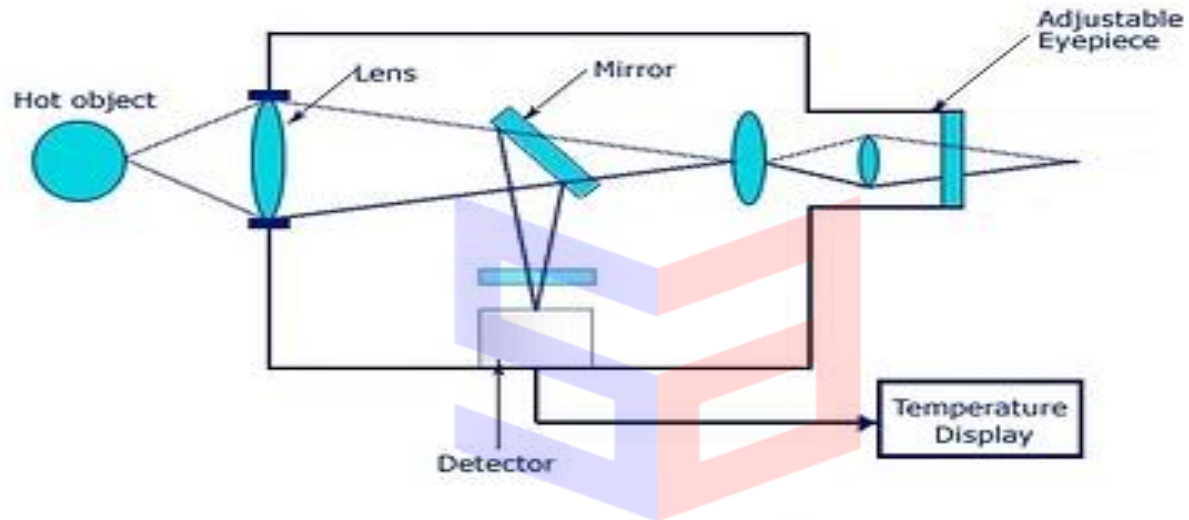
✓Radiation Pyrometer
