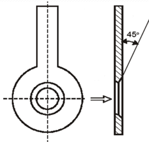
Concentric orifice plate
