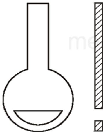
Segmental orifice plate
