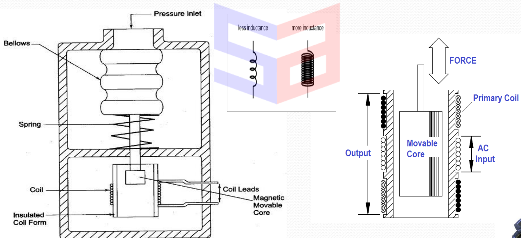
Fig. 13.22 Pressure Inductive Transducer. Sparks Academy, Ph. 81908 79379, No.16, 2F, Dharmaraja koil Street, Saidapet, Chennai - 15.
